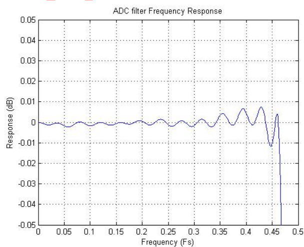
Figure 7: ADC Filter Ripple
